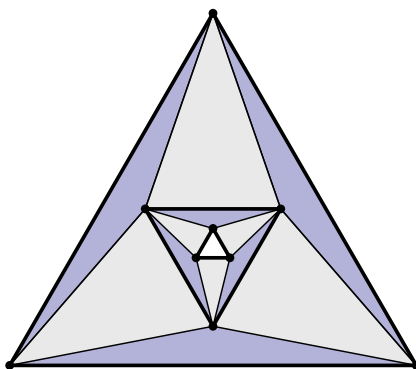
Figure 3.2: Stacking two (K_3, K_3) -transformers yields a larger a (K_3, K_3) -transformer
